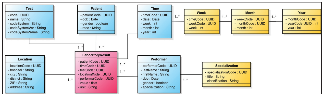
Figure 1: Example of a dimensional representing a snowflake schema composed by a Fact LaboratoryResult related to five dimensions: Test, Patient, Time, Location and Performer.
