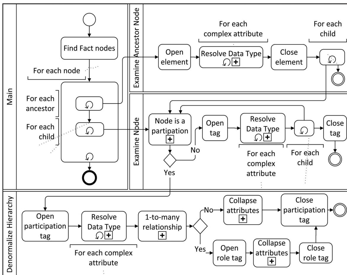
Figure 6: Business process to generate the XSLT document.
