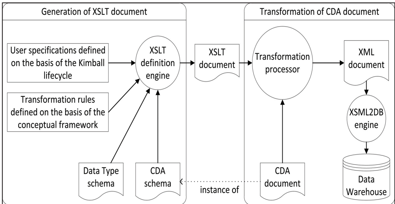
Figure 5: Transformation process to load a CDA document in a Data Warehouse.
