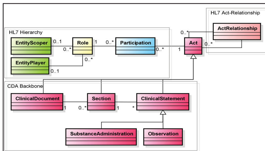
Figure 2: High level class diagram of the CDA schema modelled using the HL7 RIM core classes. The two main components of the CDA are also highlighted: 1) HL7 Hierarchy composed by the triple <Participation, Role, Entity> related to the Act class; 2) CDA Backbone defined by Act specializations and their relationships.
